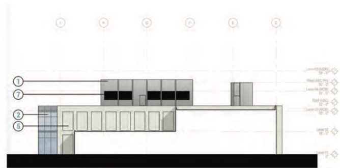
F SOUTH ELEVATION - ASC 1" = 20'
