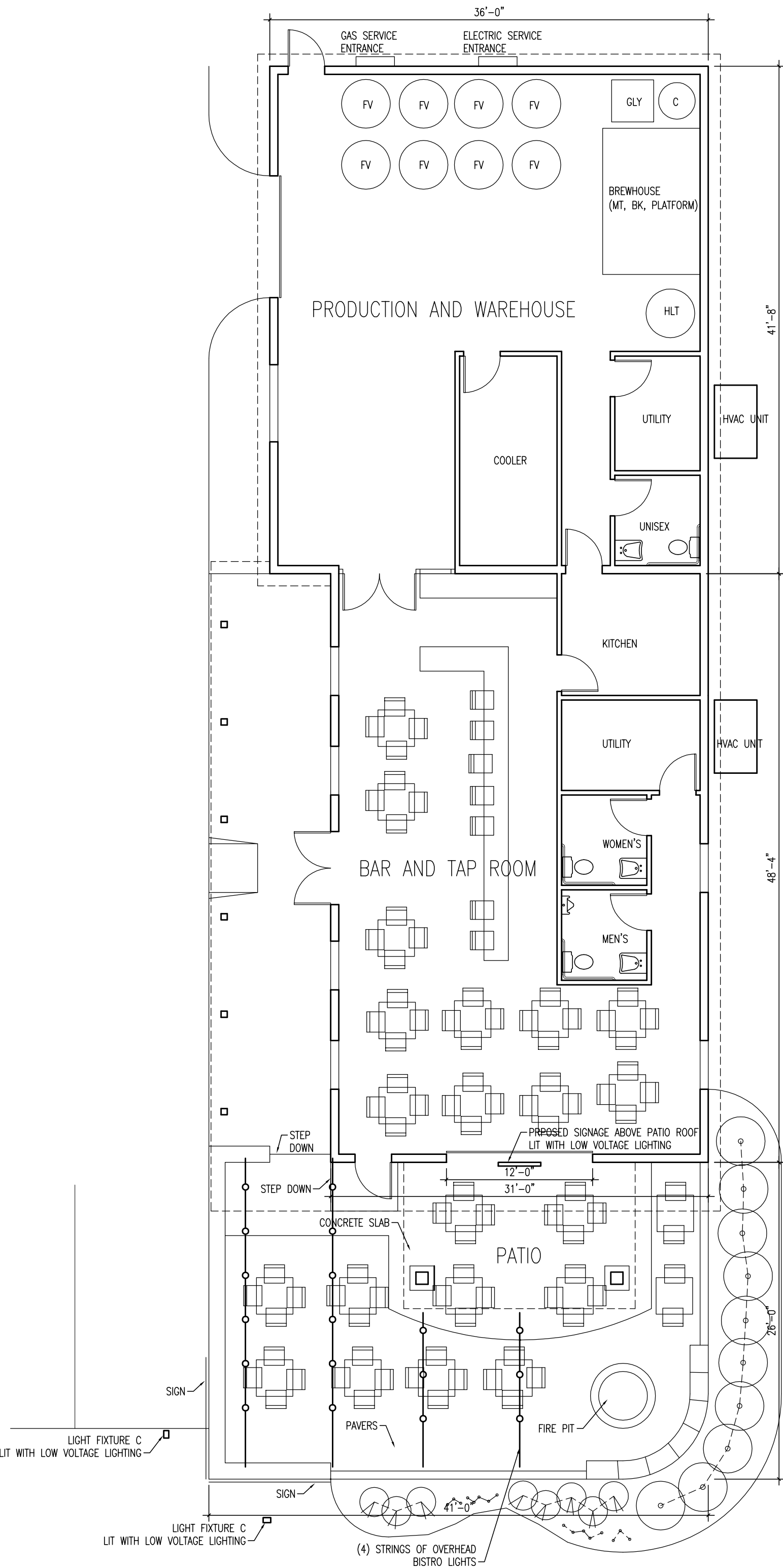
1 A-1 GRACE PLAZA ADDITION FLOOR PLAN 1/8" = 1'-0"
