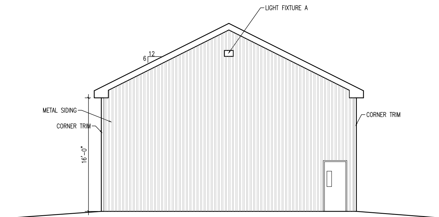
4 A-1 NORTH ELEVATION 1/8" = 1'-0"
